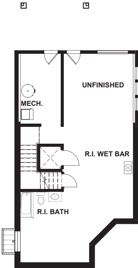
Unfinished Basement 945 SQ.FT.
